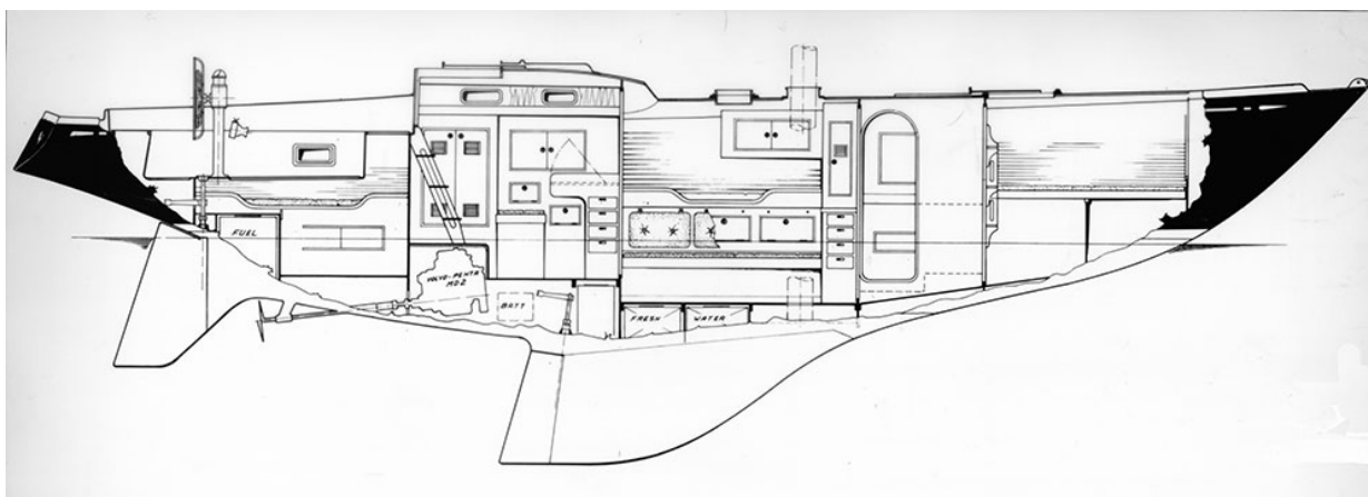
S&S Swan 43 profile
